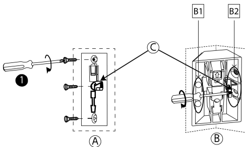
Figure 4 - Bracket Mounting
