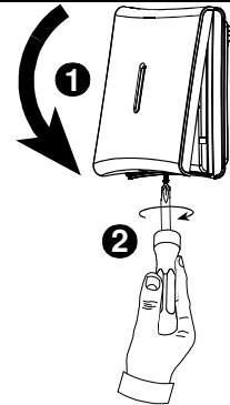
Figure 4 - Cover Closure
